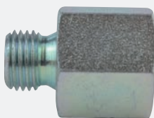
B.21.0089 Nipples 1/4" bsp female - 7/16" unf male
